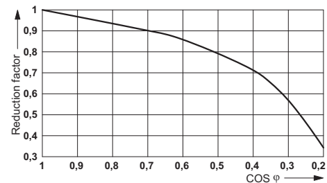
Service life reduction factor with various \cos \varphi
